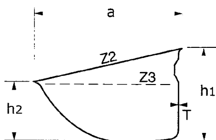
Claus elevator buckets made of plastic (parameters in mm)
